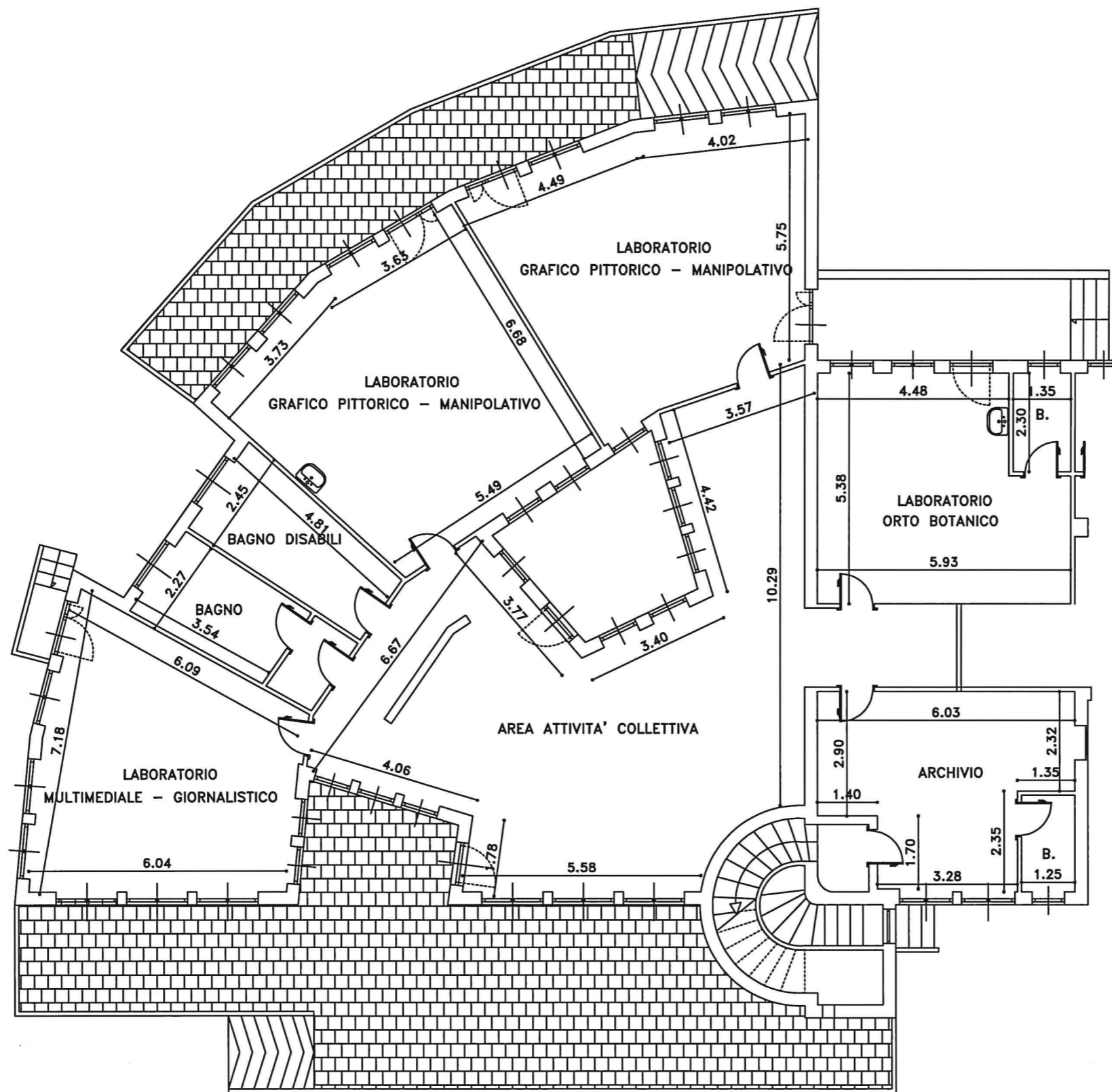
SUPERFICIE MQ.280 PIANO TERRA FACTOR URBAN LAB
